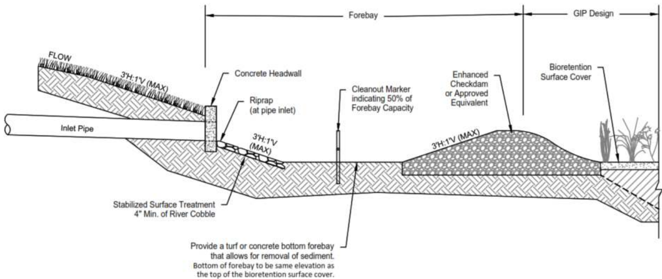
Figure 1.7: Forebay Detail
