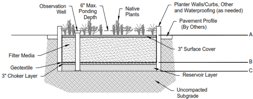
Figure 2.3. Design Details
