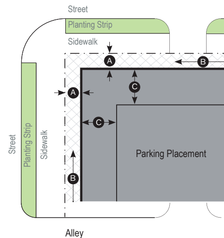
Building Plan
