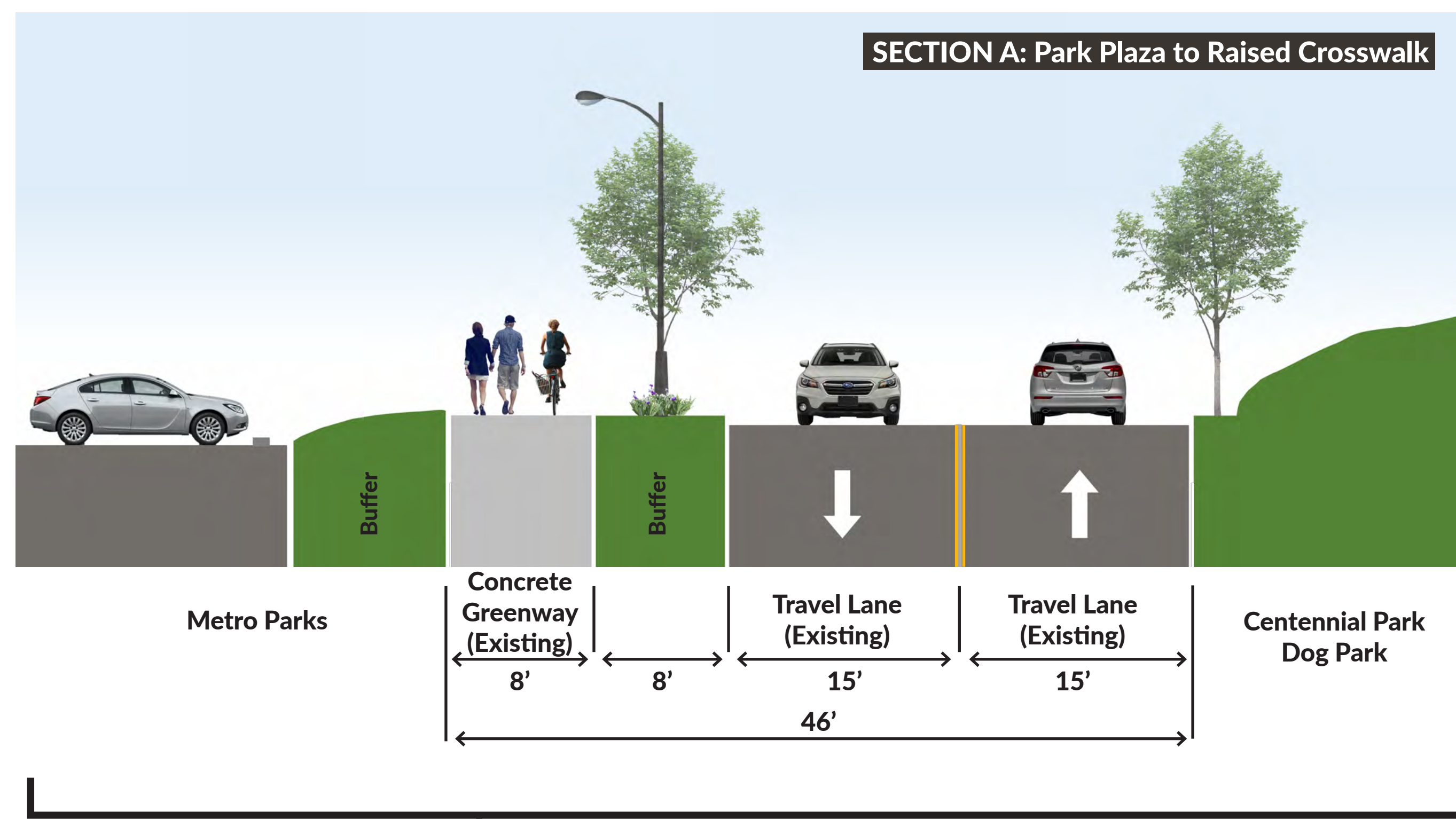
CROSS SECTION A VIEW
