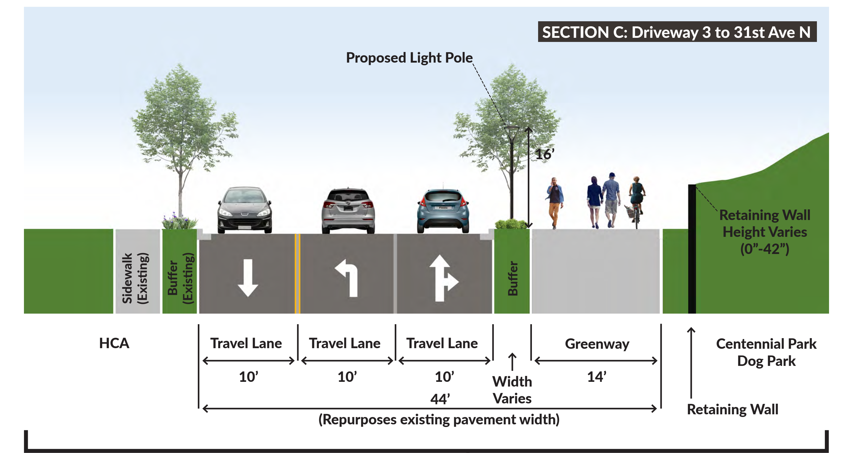
CROSS SECTION C VIEW
