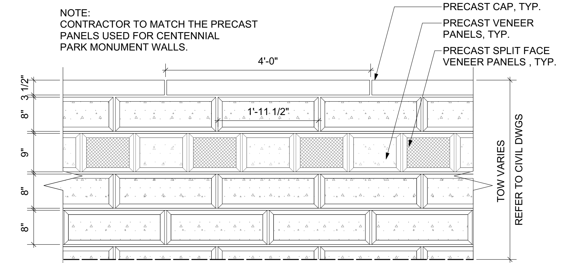
1 ELEVATION: RETAINING WALL TYP. Scale: 1" = 1'-0"
