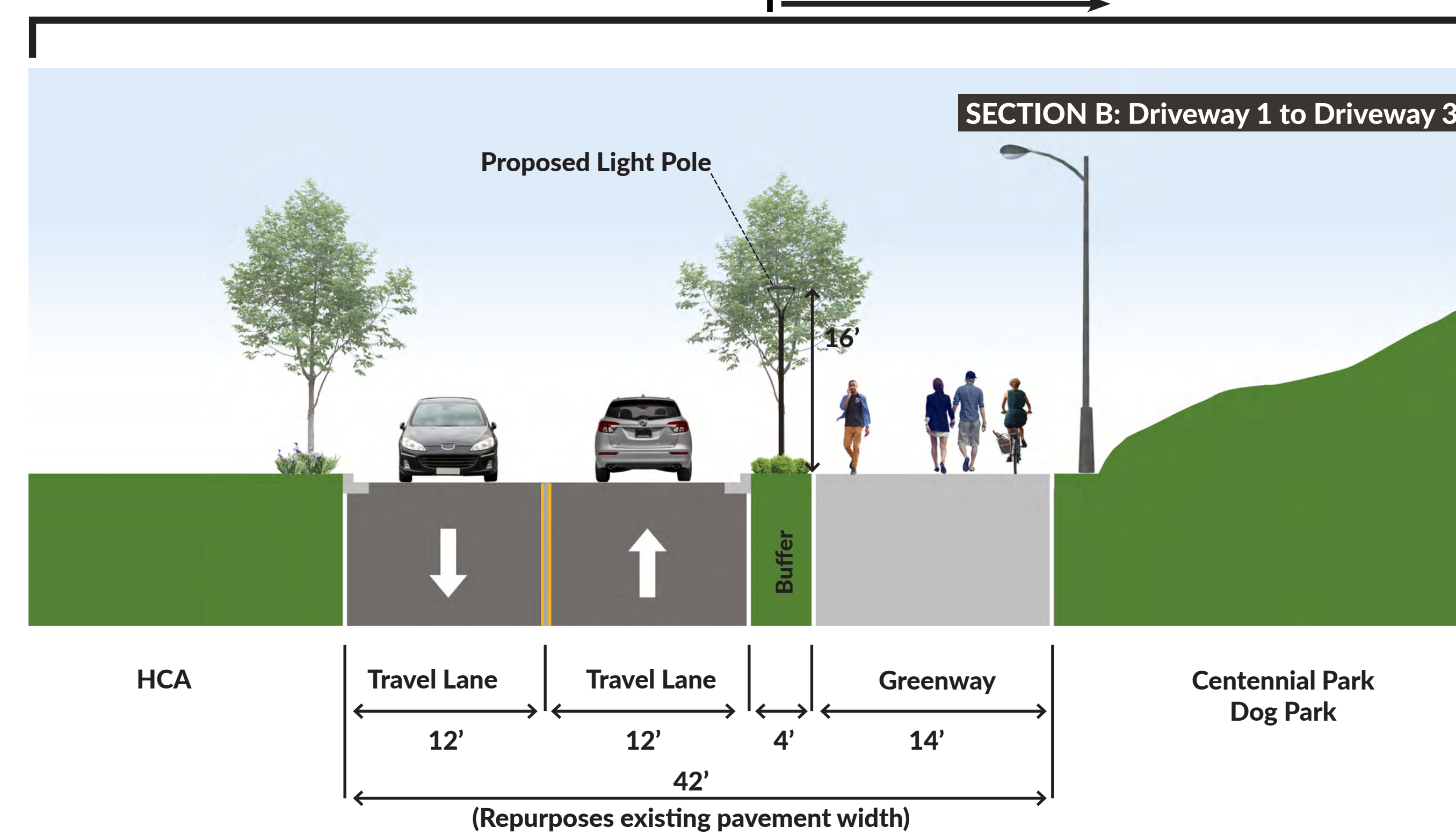
CROSS SECTION B VIEW
