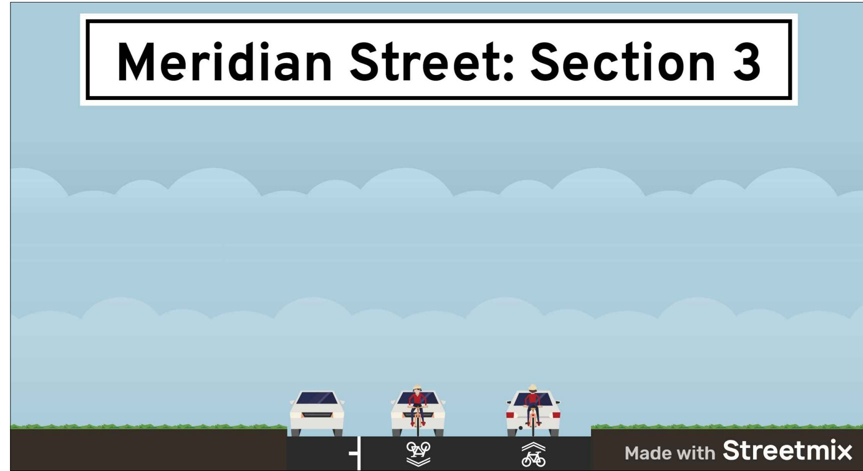
8' PARKING LANE 12.5' TRAVEL LANE WITH SHARROWS 12.5' TRAVEL LANE WITH SHARROWS
